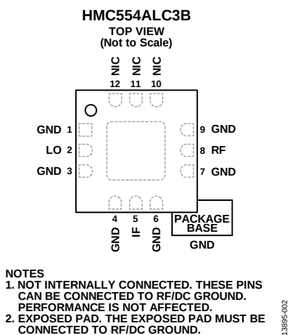
Figure 2. Pin Configuration
